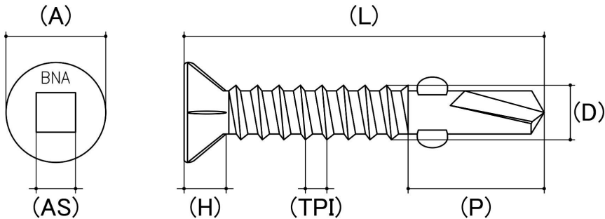
Cad Drawings shown for graphic representation only.*
